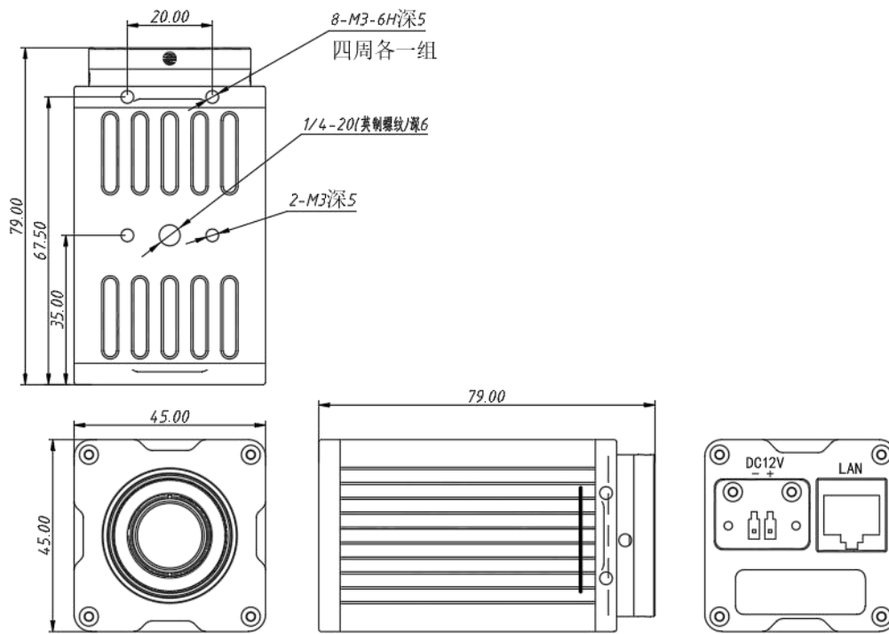
Figure 3 G43/G46 movement structure diagram
