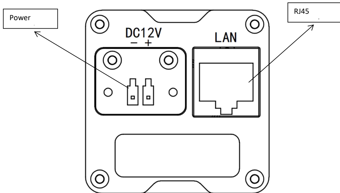
Figure 2 Interface diagram
