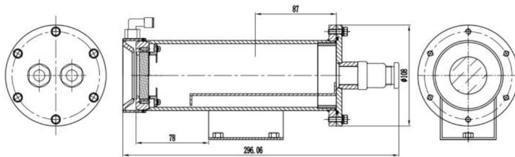
PSWExDG300-NS Structural dimensional drawing
