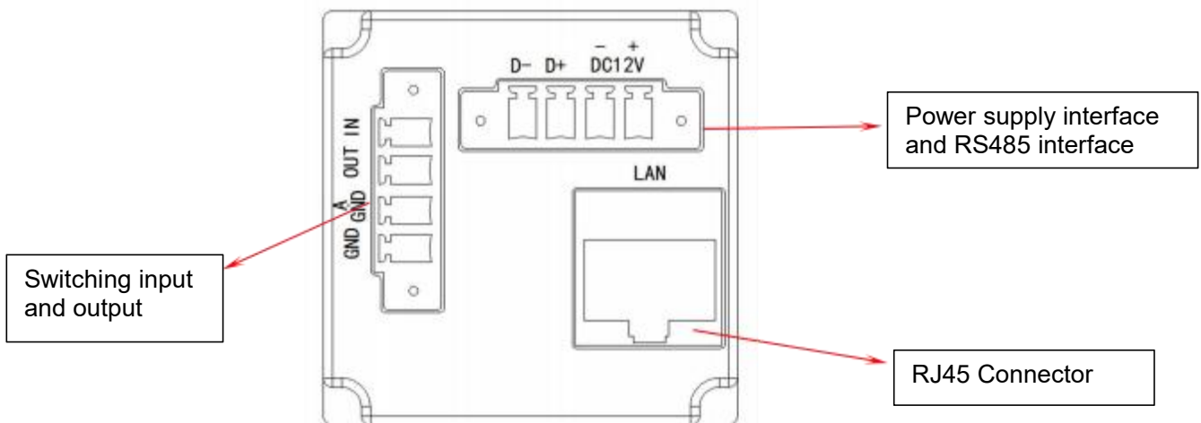
Figure 2 Interface board connector definition
