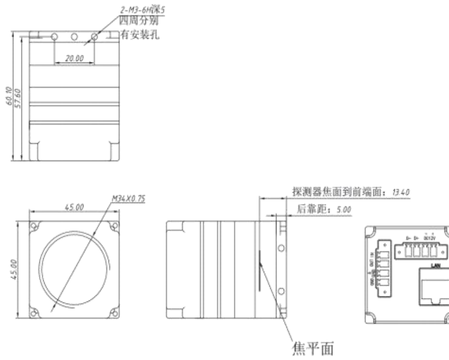
Structure and dimensions of the NX23
